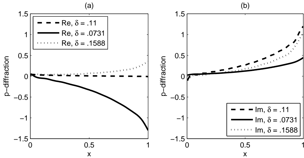
Figure 2 (a) Real and (b) imaginary parts of diffraction force on a beam, in three water depths.
