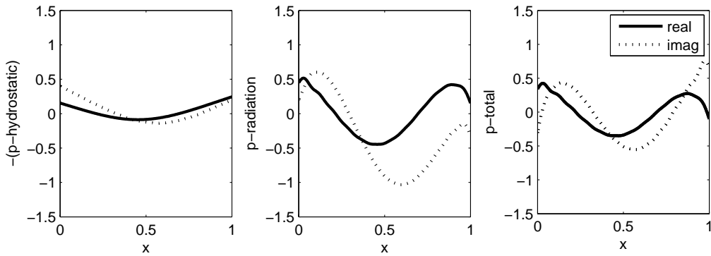
Figure 5 As for Figure 3, but with \beta = 10^3 \beta_{ref} .
