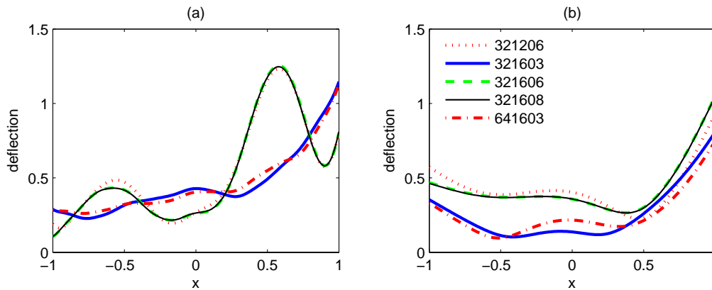
Figure 6 Modulus of deflection of square plate, calculated with different numerical models: (a) reference plate; b stiffer plate.
