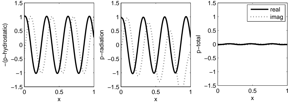
Figure 4 As for Figure 3, but with \beta = 10^{-3} \beta_{ref} .
