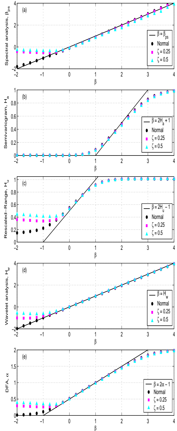
Figure 1. Scaling exponent estimates using: (a) spectral analysis; (b) semivariograms; (c) rescaled-range analysis; (d) wavelet analysis; and (e) detrended fluctuation analysis (DFA).
