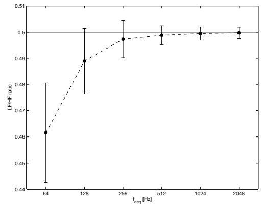
Figure 5. LF/HF ratio estimates computed from synthetic ECG signals for a range of sampling frequencies using an input LF/HF ratio of 0.5 (horizontal line). The distribution of estimates is shown by the mean (dot) and plus/minus one standard deviation error bars. The simulations used 100 realisations of noise-free synthetic ECG signals with a mean heart rate of 60 bpm and standard deviation of 3 bpm.
