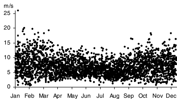
Fig. 1. Daily midday wind speed at Bears Down wind farm.
