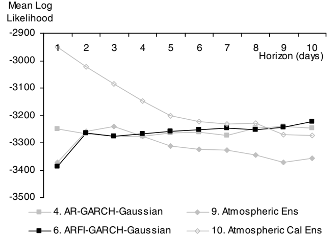
Fig. 7. Post-sample log-likelihood results averaged over the five locations.
