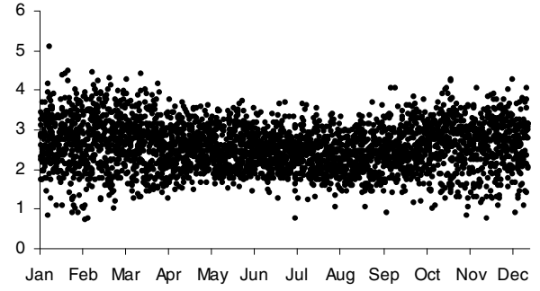
Fig. 5. Square root of daily midday wind speed observations at Bears Down wind farm plotted against the day of the year for the estimation period 1995 to 2002.
