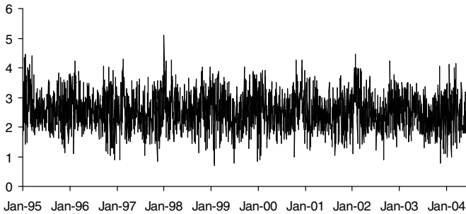
Fig. 4. Square root of daily midday wind speed at Bears Down wind farm.
